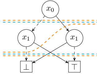
Figure 6: 1-level (cyan) and 2-level (orange) cuts in the x_0 \oplus x_1 BDD.
