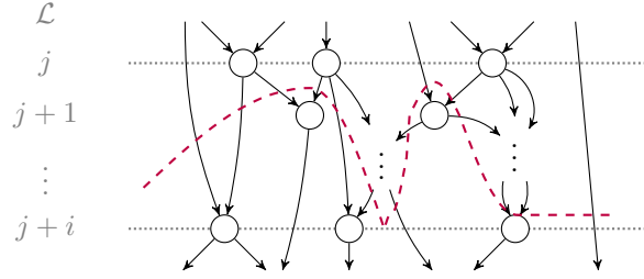
Figure 5: Visualisation of an i -level cut.
